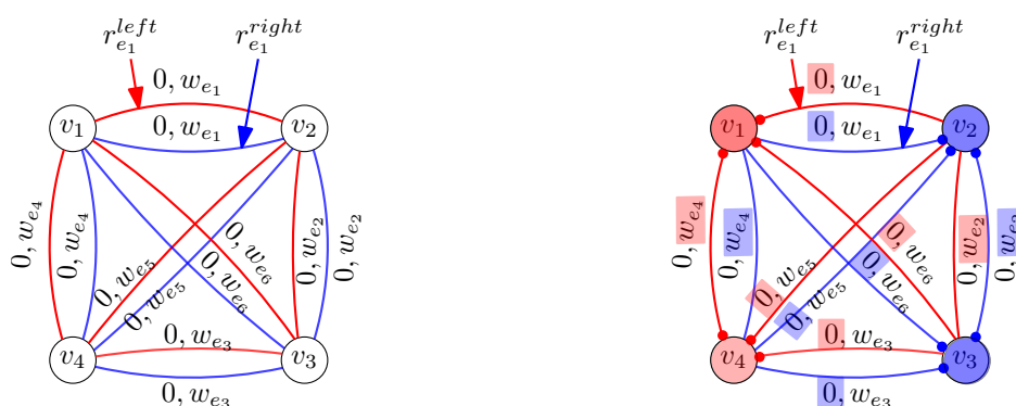
(a) The instance derived from the Max-Cut instance in Example 15.
